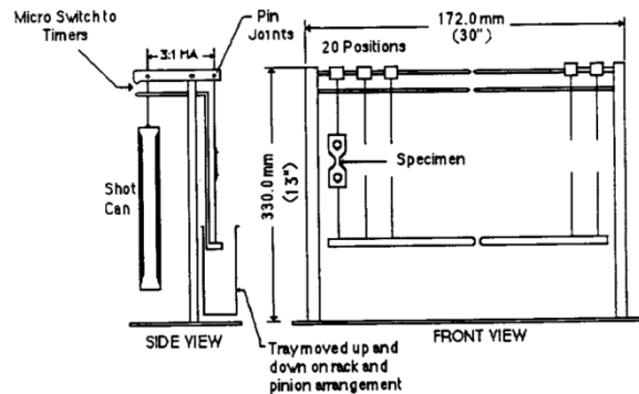
Figure 2: ASTM D5397 Test Setup
