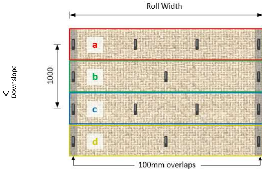
Pinning Pattern PC-3
