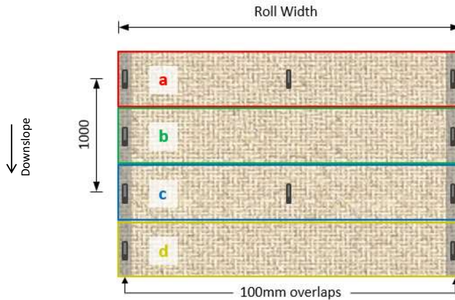
Pinning Pattern PC-2
