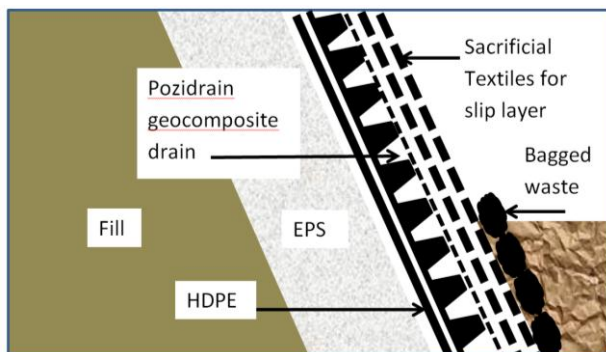
Cross section of the lining system
